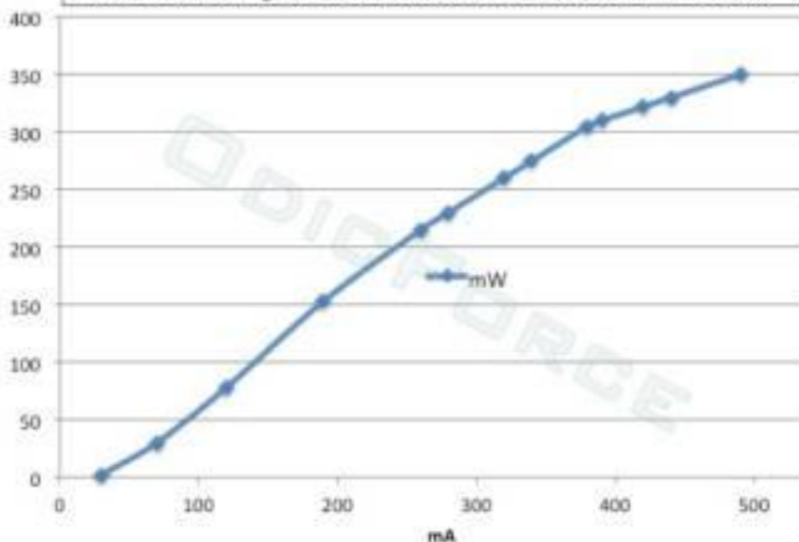
Test Data Using OFL301 LM358 Driver and OFL 177 Lens
